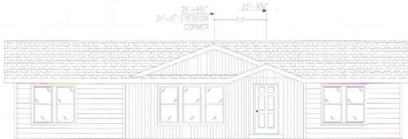
FRONT SIDEWALL WITH 24'-0" EYEBROW DORMER AND REC. ENTRY
