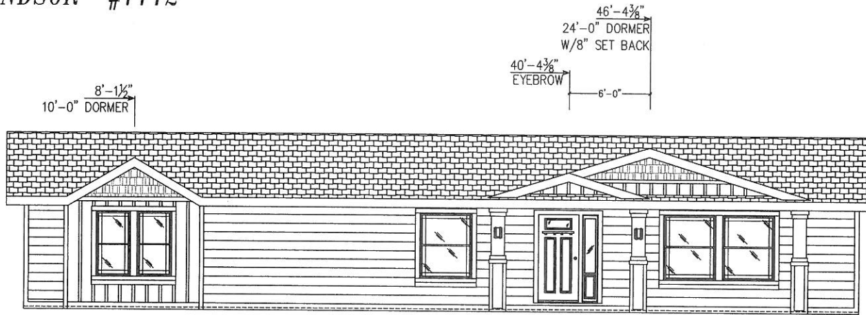
FRONT SIDEWALL
